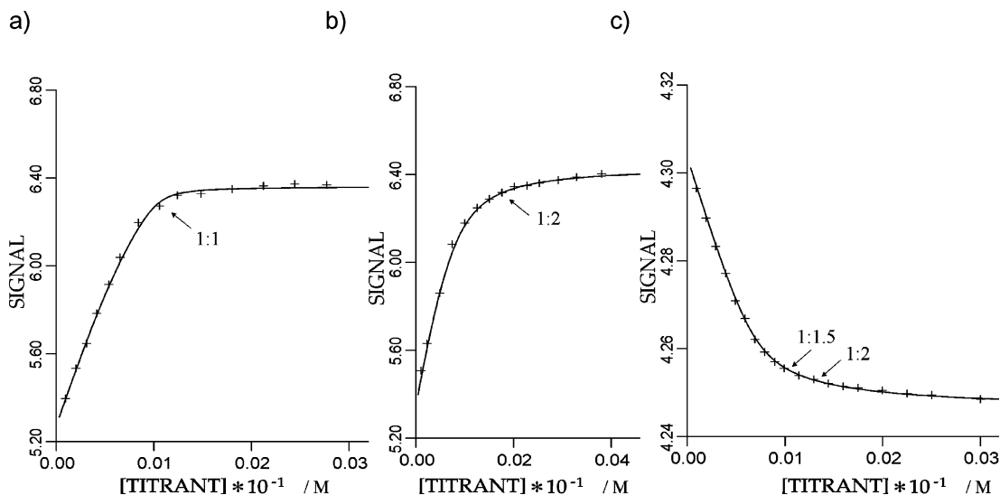
Figure 4. a, b) Plot of the observed (x) and calculated (—) chemical shifts of the amide NH signal of 1 (1.05 and 0.85 mM) as a function of added \beta -glucopyranoside 5 (a) or \alpha -glucopyranoside 6 (b); the [receptor]:[sugar] ratio is marked. c) Chemical shift changes observed for 1-CH of 5 during the titration of 5 (0.68 mM) with 1 (inverse titration); the [sugar]:[receptor] ratio is marked.
