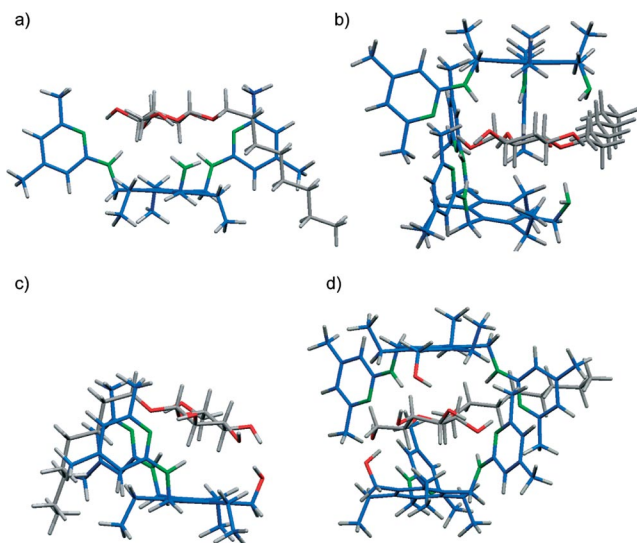
Figure 7. Energy-minimized structure of a) the 1:1 complex formed between receptor 2 and \beta -glucopyranoside 5 , b) the 2:1 receptor–sugar complex between 2 and 5 , c) the 1:1 complex between receptor 3 and \beta -glucopyranoside 5 , and d) the 2:1 receptor–sugar complex formed between 3 and 5 (MacroModel V.8.5, OPLS-AA forcefield, MCMM, 50000 steps). Color code: receptor C, blue; receptor N, green; sugar O, red; sugar C/H, grey.
