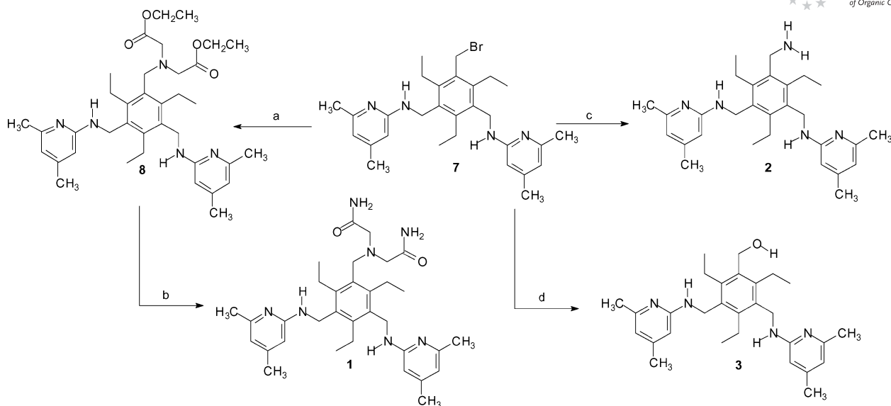
Scheme 1. a) \text{HN}(\text{CH}_2\text{COOCH}_2\text{CH}_3)_2 , THF/ \text{CH}_3\text{CN} , \text{K}_2\text{CO}_3 , 24 h, yield 60%; b) \text{NH}_3/\text{CH}_3\text{OH} , 48 h; yield 39%; c) \text{NH}_3/\text{H}_2\text{O} (25% solution), THF/ \text{CH}_3\text{OH} , 12 h; yield 72%; d) NaOH aq., THF, 5 h; yield 75%.
