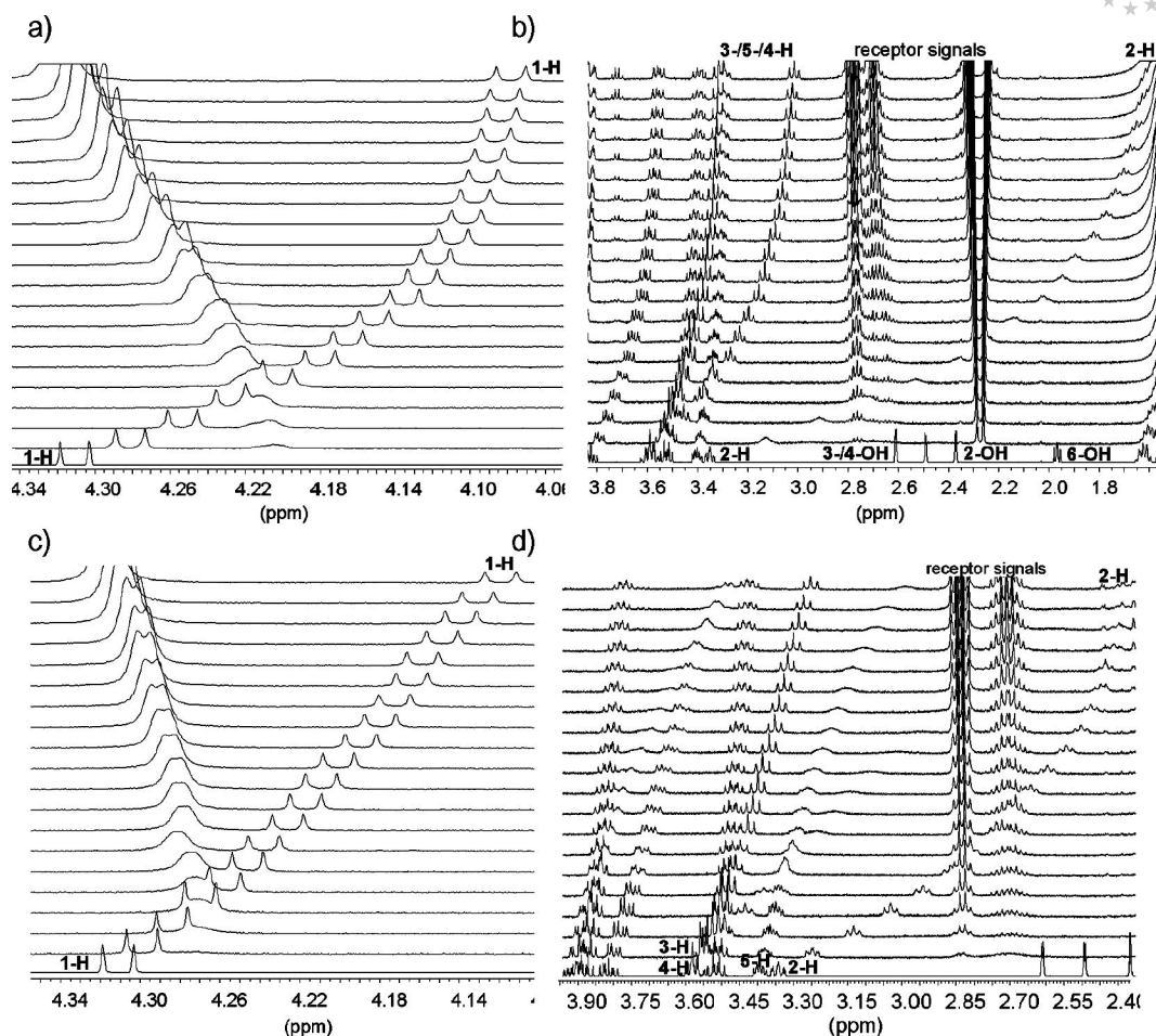
Figure 6. a, b) Partial ^1\text{H} NMR spectra (500 MHz, \text{CDCl}_3 ) of \beta -glucopyranoside 5 after addition of (from bottom to top) 0.00–4.94 equiv. of 2 ( [\mathbf{5}] = 0.69 mM). c and d) Partial ^1\text{H} NMR spectra (500 MHz, \text{CDCl}_3 ) of \beta -glucopyranoside 5 after addition of (from bottom to top) 0.00–4.91 equiv. of 3 ( [\mathbf{5}] = 0.70 mM).
