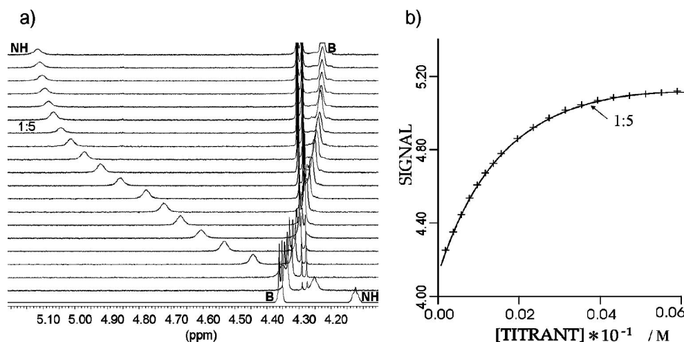
Figure 8. a) Partial 1 H NMR spectra (500 MHz, CDCl 3 ) of 4 after addition of (from bottom to top) 0.00–7.42 equiv. of β-glucopyranoside 5 ([ 4 ] = 0.80 mM). Shown are chemical shifts of the CH 2 B and NH A resonances of 4 (for labelling, see Figure 4). b) Plot of the observed (×) and calculated (–) chemical shifts of the NH A signal of 4 as a function of added 5 .
