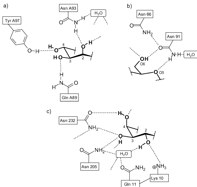
Figure 1. Examples of hydrogen bonds in the complexes of: a) Galanthus nivalis lectin with mannose, [3f,3a] b) D-galactose-binding protein with D-glucose, [3b] and c) L-arabinose-binding protein with L-arabinose. [3b]
