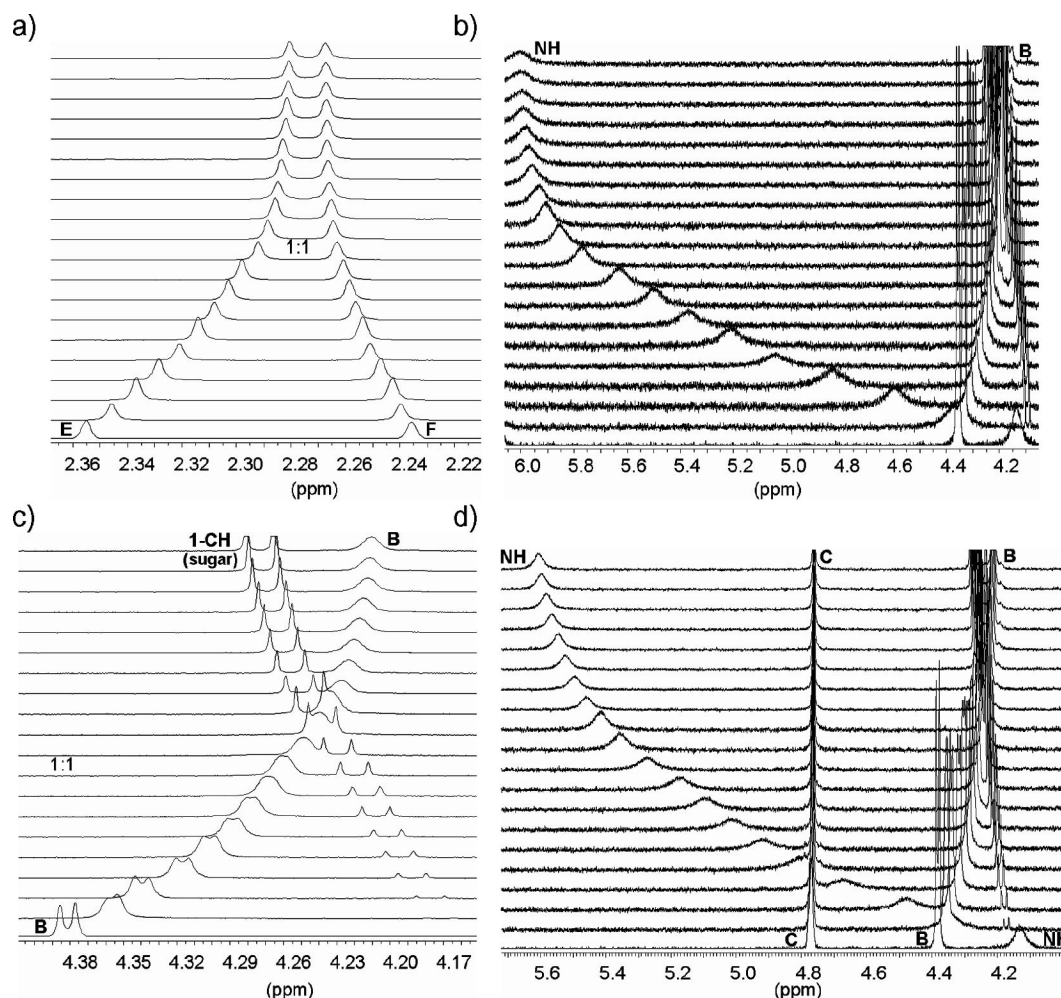
Figure 5. a, b) Partial ^1\text{H} NMR spectra (500 MHz, \text{CDCl}_3 ) of 2 after addition of (from bottom to top) 0.00–3.55 equiv. of \beta -glucopyranoside 5 ( [\text{2}] = 0.99 \text{ mM} ). Shown are chemical shifts of the \text{CH}_3^{\text{E,F}} and \text{NH}^{\text{A}} resonances of 2 (for labelling, see Figure 2). c, d) Partial ^1\text{H} NMR spectra of 3 after addition of (from bottom to top) 0.00–3.52 equiv. of 5 ( [\text{3}] = 0.99 \text{ mM} ). Shown are chemical shifts of the \text{CH}_2^{\text{B,C}} and \text{NH}^{\text{A}} resonances of 3 .
