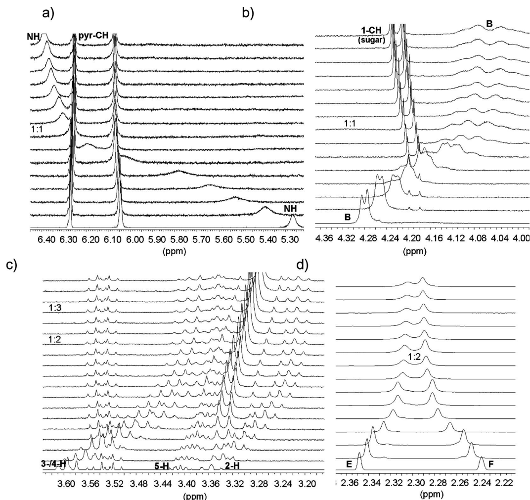
Figure 3. a, b) Partial ^1\text{H} NMR spectra (400 MHz, \text{CDCl}_3 ) of 1 after addition of (from bottom to top) 0.00–3.03 equiv. of \beta -glucopyranoside 5 ( [\mathbf{1}] = 1.00 mM). Shown are chemical shifts of the amide NH and \text{CH}_2^{\text{B}} resonances of 1 (for labelling, see formula 1 ). c) Partial ^1\text{H} NMR spectra (500 MHz, \text{CDCl}_3 ) of \beta -glucopyranoside 5 after addition of 0.00–4.39 equiv. of 1 ( [\mathbf{5}] = 0.68 mM). Shown are chemical shifts of the CH-2, -3, -4 and CH-5 resonances of 5 (as well as shifts of the OCH proton of 5 ). d) Partial ^1\text{H} NMR spectra (400 MHz, \text{CDCl}_3 ) of receptor 1 after addition of 0.00–4.95 equiv. of \alpha -glucopyranoside 6 ( [\mathbf{1}] = 0.85 mM). Shown are chemical shifts of the \text{CH}_3^{\text{E,F}} resonances of 1 .
