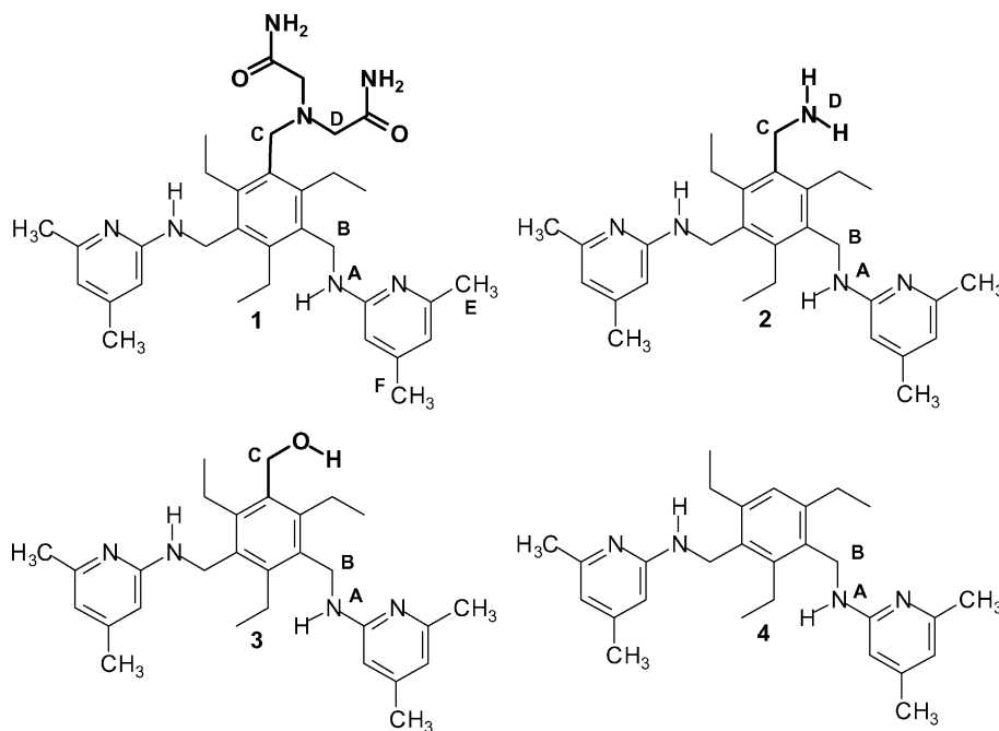
Figure 2. Structures of receptors 1–4.
